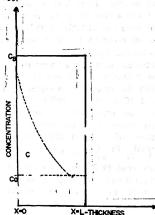
Fig. 1: Variation of hydrogen concentration ( C ) along the thickness of a thin slab (thickness of slab = L ). C_0 is the initial concentration (distributed uniformly) of hydrogen in the slab. C_s is the concentration of the hydrogen atmosphere into which the absorbing face (face at X=0 ) of the slab is exposed.
