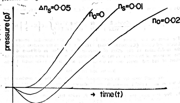
Fig. 2: Variation with time ( t ) of the pressure ( P ) inside the volume V (into which the diffused hydrogen atoms are being collected) computed using equation (8) with \Delta n_s=0.05 and different values for n_0
